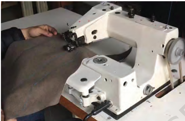
Fig. 1.12: Blind stitch machine
